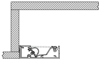
Architectural Cove 4" minimum offset, 12" typical offset. Can be installed in Cove or Coffer.
