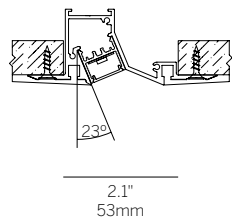
Gypsum Wall
