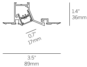
Recessed Plaster Trim (RPT)
