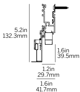
Recessed Grid Trim (RGT9/RGT15)
