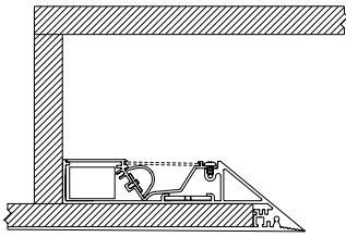
Gypsum Ceiling Mounting 4" (100mm) minimum offset, 12" (305mm) typical offset Can be installed in Cove or Coffered
