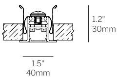
Solid Ceiling Mounting Options
