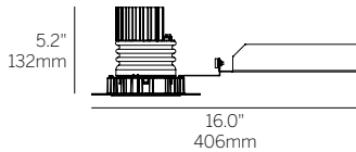
Recessed Bezel Trim
