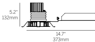
Recessed Plaster Trim (RPT)
