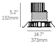
Recessed Plaster Trim (RPT)
