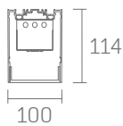
surface mount
