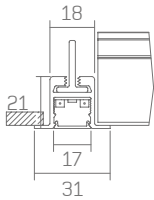
Grid Ceiling
