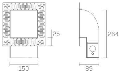
Plaster-in
