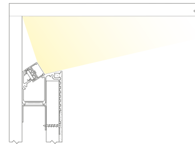
Concealed ceiling wash from wall pocket
