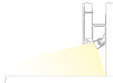
Concealed floor wash from wall pocket
